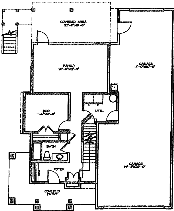
LOWER FLOOR PLAN 789 SQ. FT.
