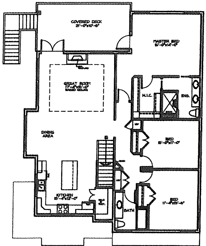
MAIN FLOOR PLAN 1644 SQ. FT. 2433 SQ. FT. TOTAL.
